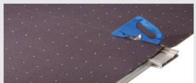
USF rail in use with electric circular knife USM-G and carpet cutters
