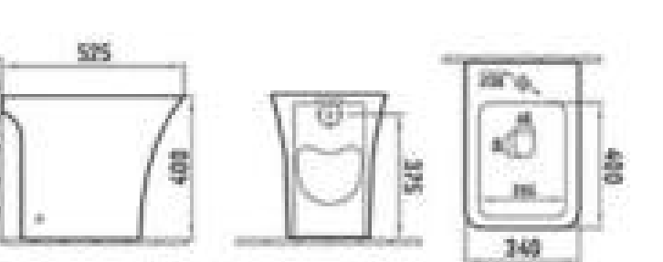
3101-B2971B Bidet Size: 525x340x400mm
