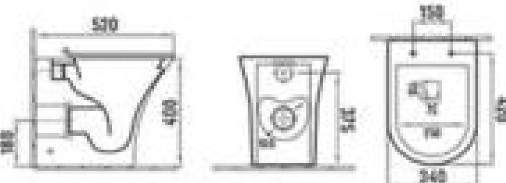
3095-LB2970B Back-to-wall toilet Size: 520x340x400mm P-trap: 180mm Roughing-in
