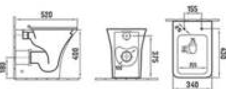
3090LB2971B Back-to-wall toilet Size: 520x340x400mm P-trap: 180mm Roughing-in
