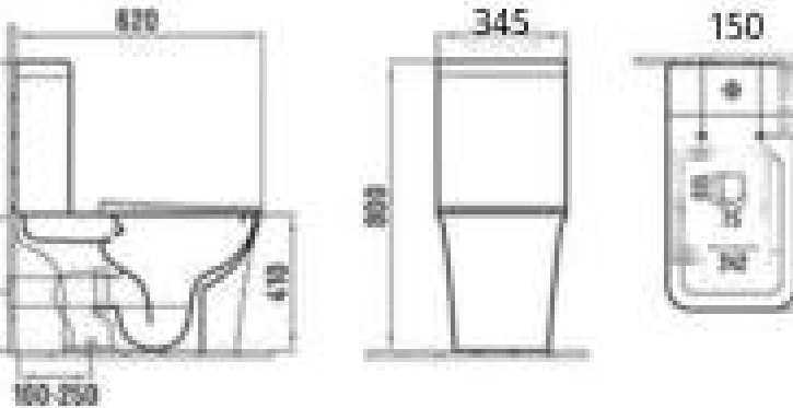
31022972 Washdown two-piece toilet Full back to wall Size: 620x345x800mm S-trap: 250mm Roughing-in P-trap: 180mm Roughing-in
