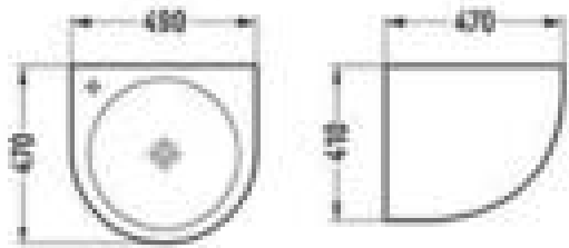
500FMH Wall-hung basin Size: 490x470x410mm Fixing to wall with back
