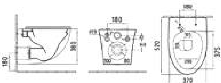
B2352 Wall-hung toilet Size: 520x370x360mm P-trap: 180mm Roughing-in
