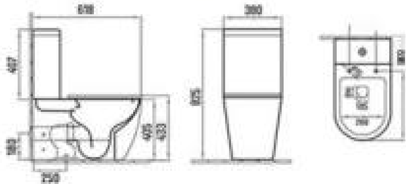
A 2342 Washdown two piece toilet. Size: 618x380x825mm S-trap 250mm Roughing-in P-trap 180mm Roughing-in
