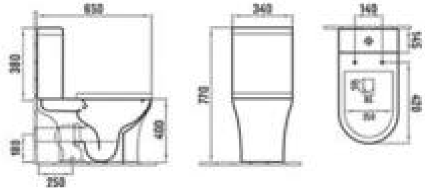
3096-2970 Washdown two-piece toilet Size: 650x340x770mm S-trap: 250mm Roughing-in P-trap: 180mm Roughing-in
