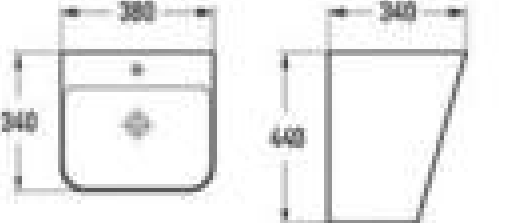
500Q Wall-hung basin Size: 380x340x440mm Fixing to wall with back
