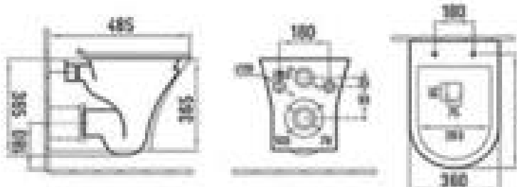
3096-B2970 Wall-hung toilet Size: 485x380x665mm P-trap: 180mm Roughing-in
