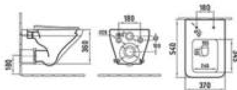
B2353 Wall-hung toilet Size: 540x370x360mm P-trap: 180mm Roughing-in
