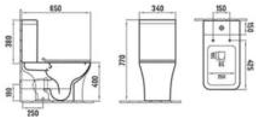
3098-2971 Washdown two-piece toilet Size: 650x340x770mm S-trap: 250mm Roughing-in P-trap: 180mm Roughing-in
