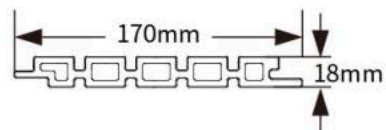
Product Cross-section 产品横截面
