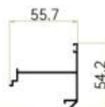
JH-PK5010 假中梃 | Dummy Intermediate Mullion 壁厚THK: 1.4 MM 米重W/M: 0.536 KG/M
