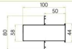
JH-PK1002 配压线JH-PK5009 加强中梃 | Reinforced Intermediate Mullion 壁厚THK: 1.2 MM 米重W/M: 1.130 KG/M
